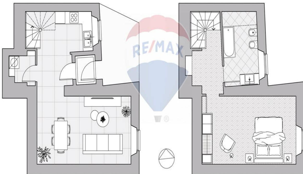
PIANO TERRA
